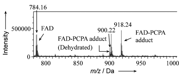
Figure 5. Mass spectrometric detection of FAD PCPA adducts. Mass spectra were obtained from LSD1/ 1a mixture (negative mode).
